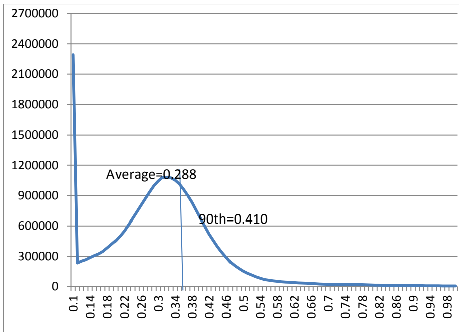
Figure 5.4.4: Response Times Frequency Distribution for Delivery Transactions
