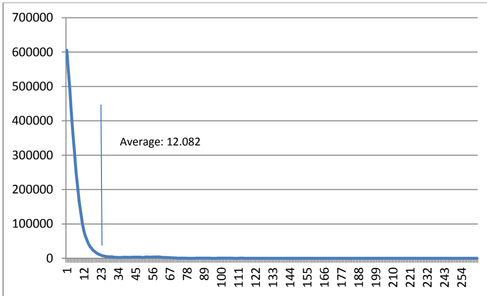
Figure 5.4.7: Think Times distribution for New Order Transactions
