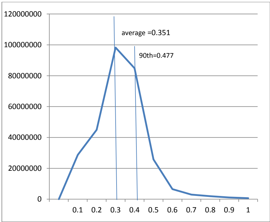
Figure 5.4.1: Response Times Frequency Distribution for New Order Transactions
