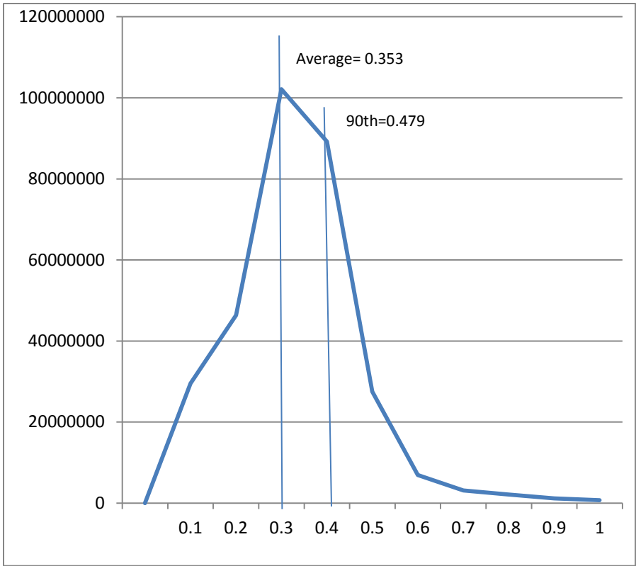
Figure 5.4.1: Response Times Frequency Distribution for New Order Transactions
