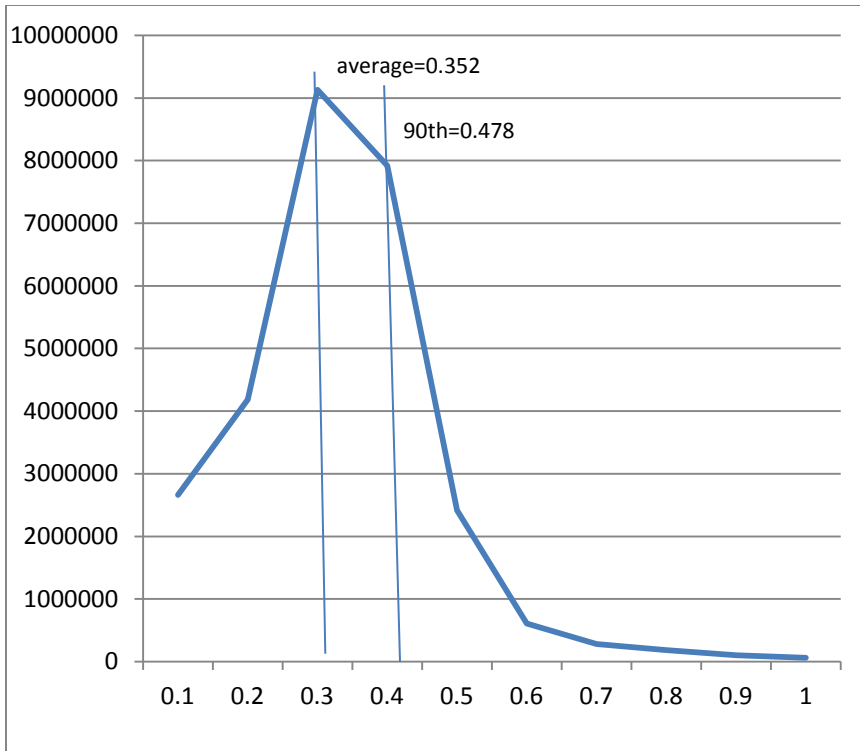
Figure 5.4.3: Response Times Frequency Distribution for Order Status Transactions
