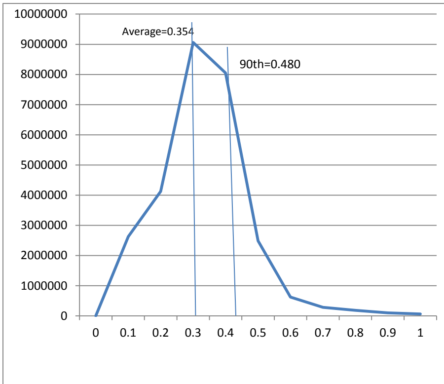
Figure 5.4.5: Response Times Frequency Distribution for Stock Level Transactions
